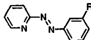
(21) R = H; (22) R = Me
