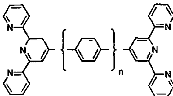
( 10 ) n = 0 ; ( 11 ) n = 1 ; ( 12 ) n = 2
